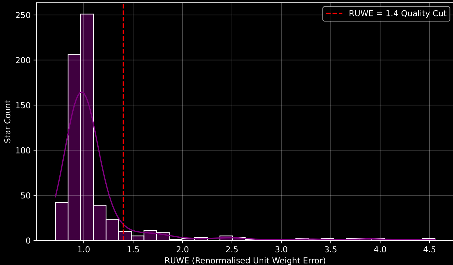
GAPOGEE DR17 Field [K07_075+17] RUWE Distribution (n= 628)
