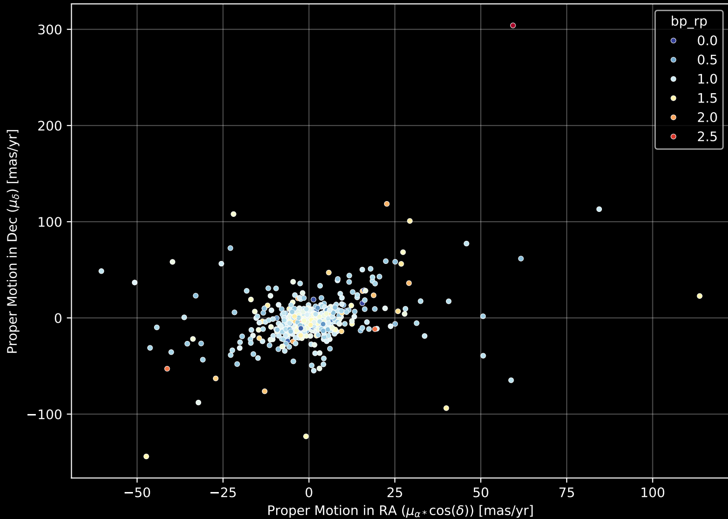
APOGEE DR17 Field: [K07_075+17] Proper Motion Diagram (n= 651)
