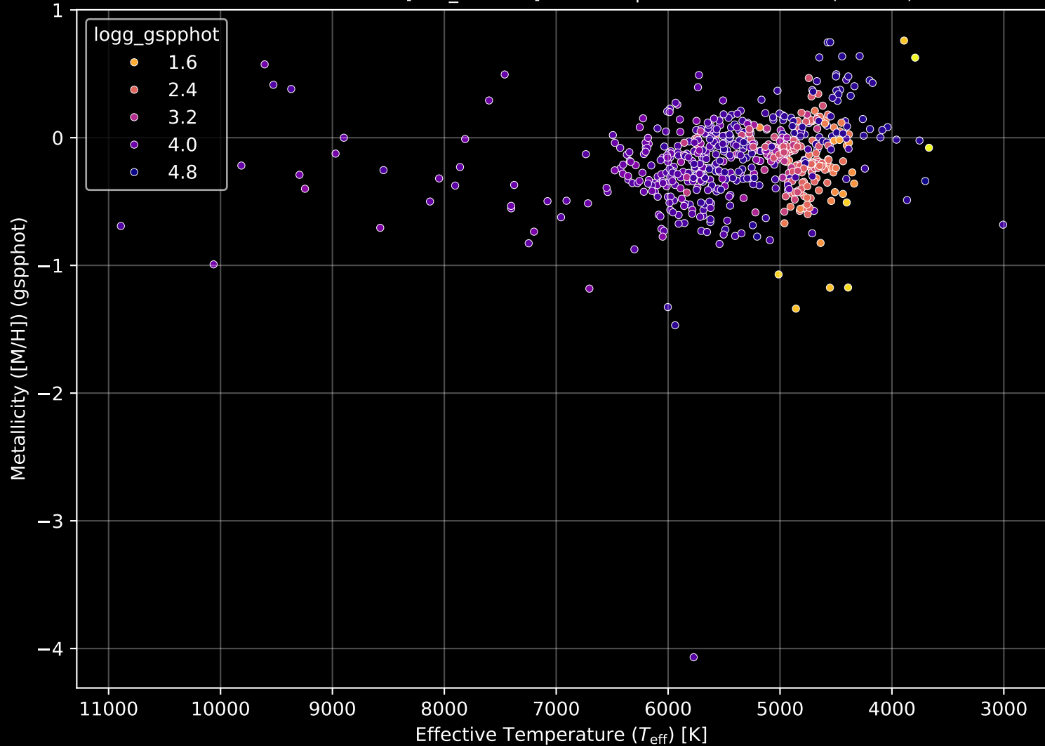
APOGEE DR17 Field: [K07_075+17] Stellar Population Parameters (n= 651)
