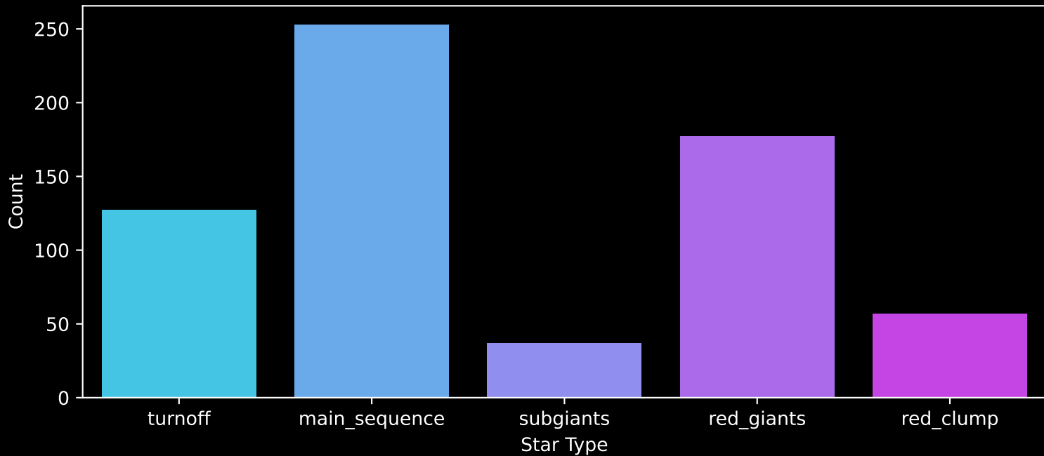
APOGEE DR17 Field: [K07_075+17] Count plot of Star Type
