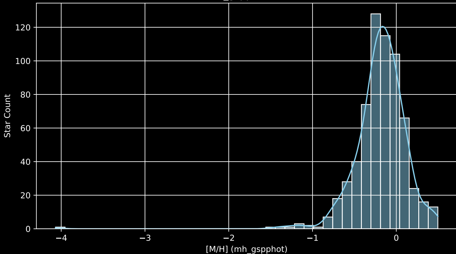
APOGEE DR17 Field: [K07_075+17] [M/H] (mh_gspphot) (n= 643)
