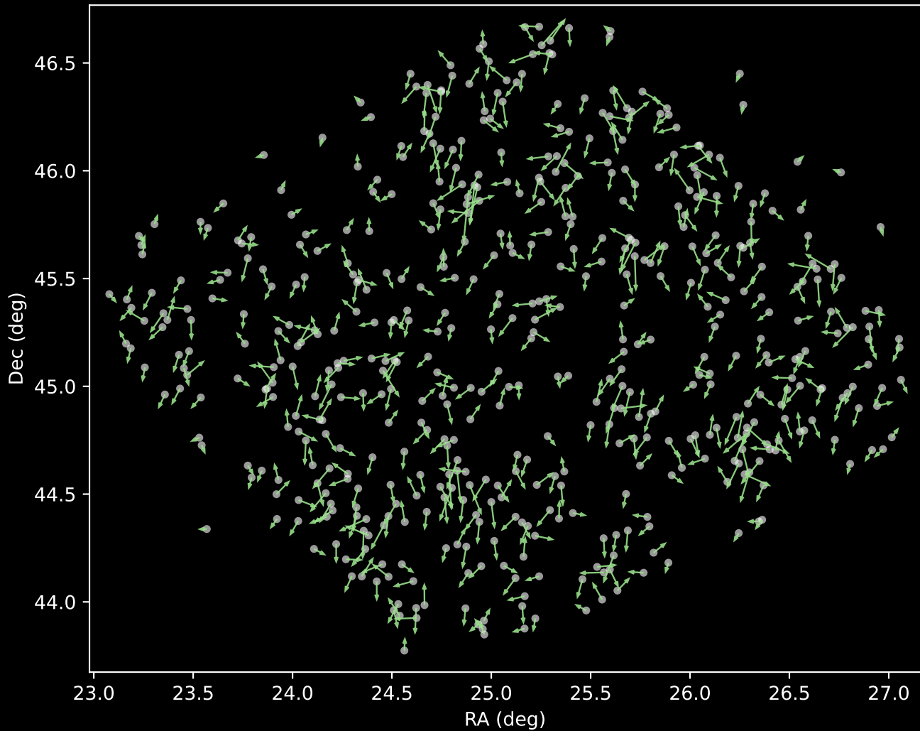
APOGEE DR17 Cluster 5 Proper Motion Vectors (n=529)
