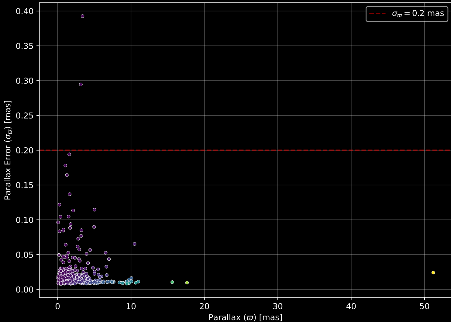
APOGEE DR17 Field: [K07_075+17] Parallax Quality (n= 651)
